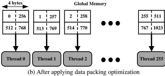
Figure 8: An example of how the data packing optimization reduces the number of global memory accesses.
