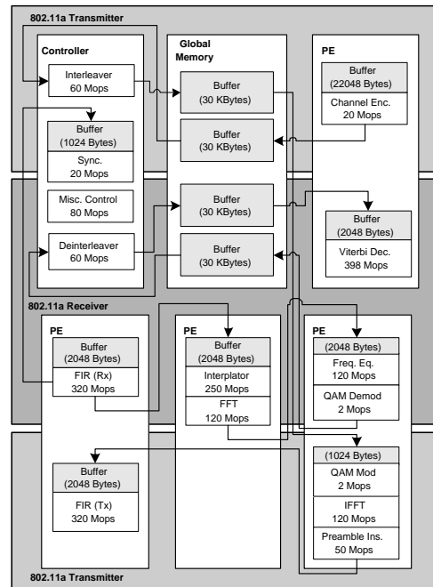
(b) 802.11a Protocol Mapping
